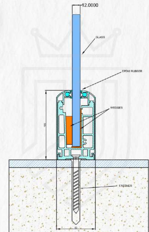
JVL-BKT-06 ROUNDED
