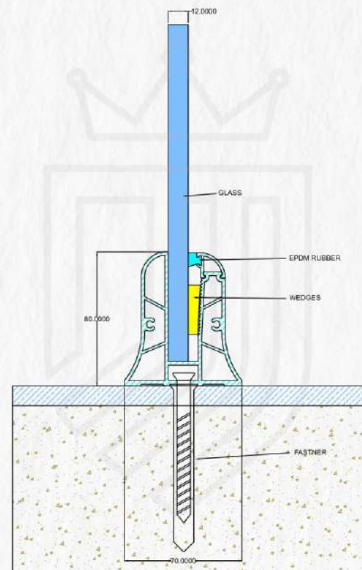
JVL-CP-11 TURKEY
