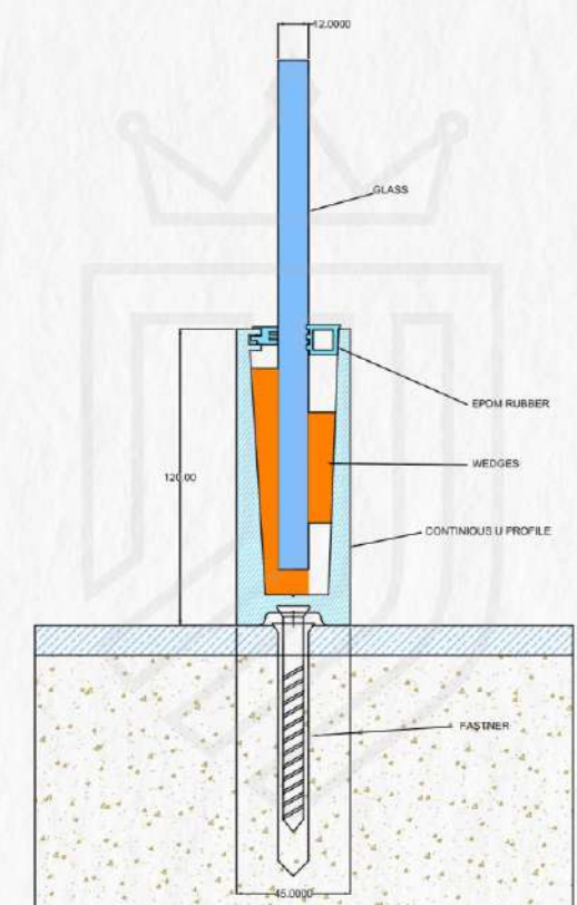
JVL-CP-08 120X45MM
