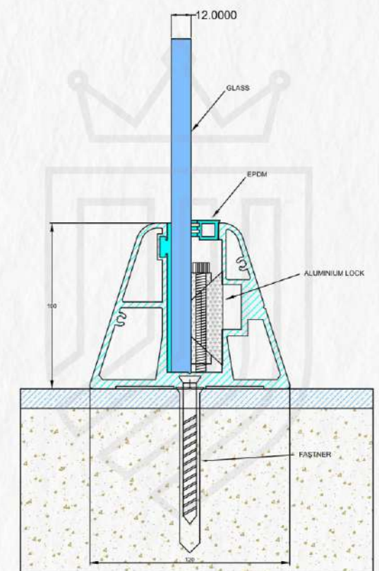
JVL-CP-18 100X120MM
