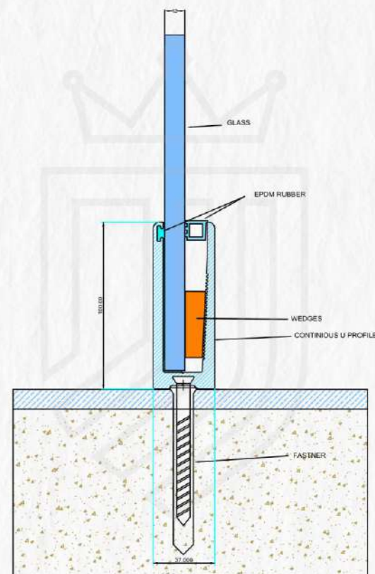
JVL-CP-07 100X37MM
